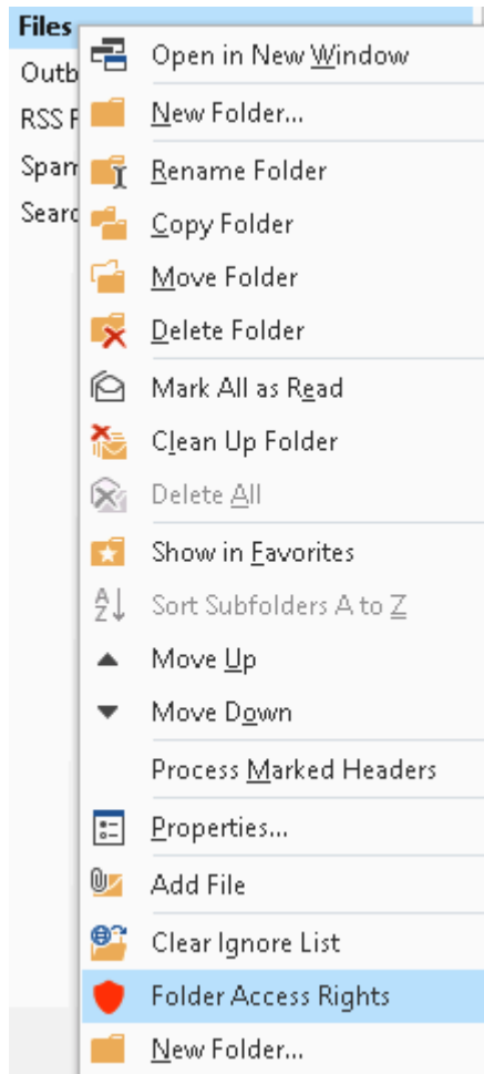
Figure 1 – Right-click Menu
